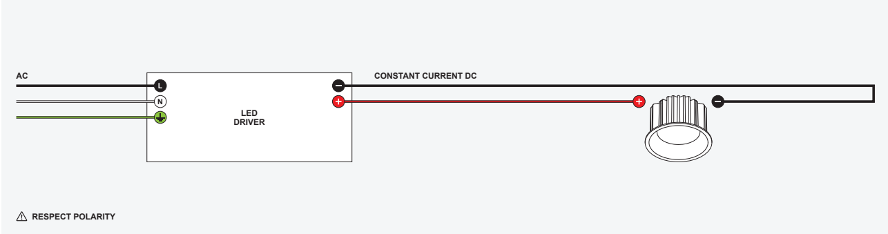
1 LED LUMINAIRE (POWERED BY A CONSTANT CURRENT LED DRIVER)
