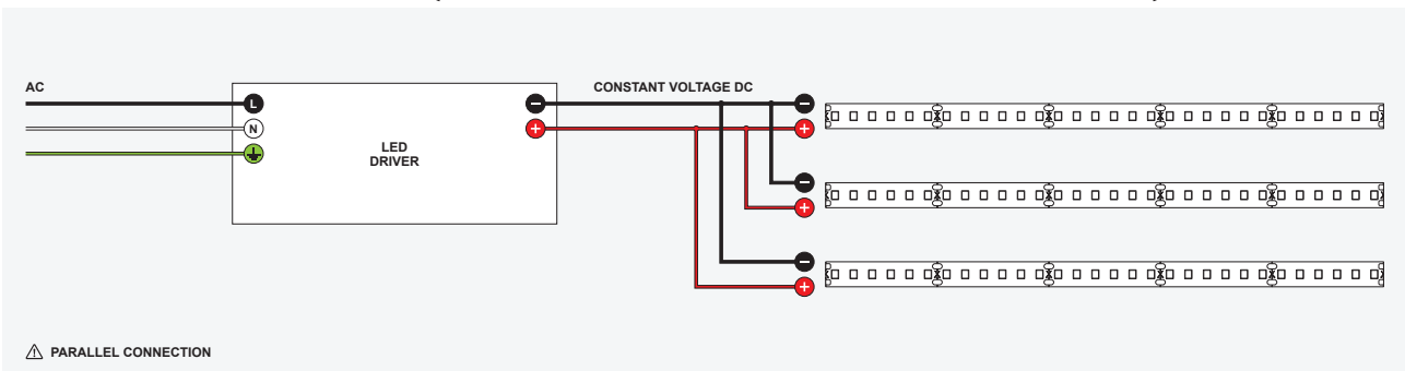
2 OR MORE LED LUMINAIRES (POWERED BY A CONSTANT VOLTAGE LED DRIVER)
